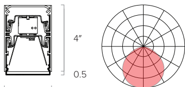
2.25" 0.5" 0.5" Drop Lens
