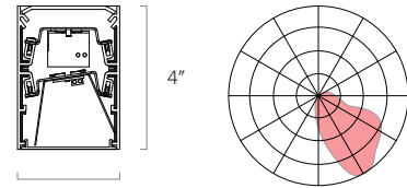
2.25" Asymmetric
