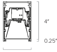
2.25" 0.25" Regressed Lens
